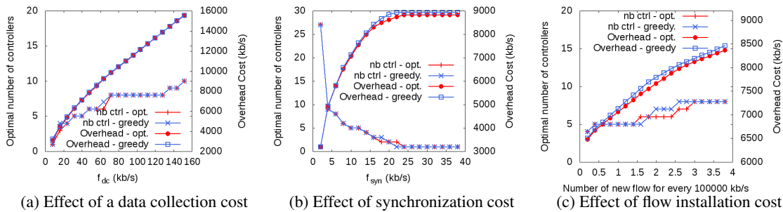
FIGURE 2: Effect of a flow installation cost on the overhead cost and the number of controllers on the GEANT topology
