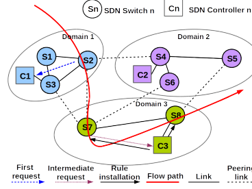
FIGURE 1: Flow requests and installations in distributed SDN networks.
