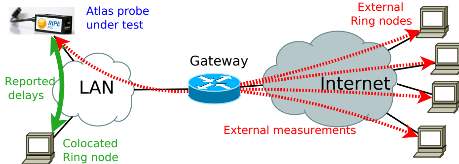
FIGURE 1: We load the probe with traceroutes and pings to distant targets while we measure the delay toward local destinations.
