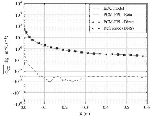
Fig. 8. Comparison of the profiles of CO mean source term obtained with various models. The black dots (●) correspond to the reference case, directly obtained from the DNS. Note that a closer comparison between Beta and Dirac approaches is shown in Fig. 14.
