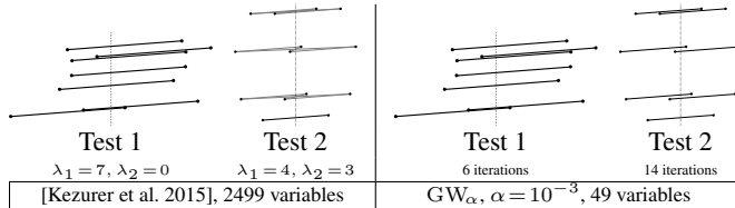
Figure 12: Comparison to SDP matching. The points on the left of the vertical dotted lines are mapped to the right; edge darkening indicates value of \Gamma . The two largest eigenvalues are shown for [Kezurer et al. 2015]; the second test case is not tight. The number of iterations for six digits of precision is shown for \text{GW}_\alpha .
