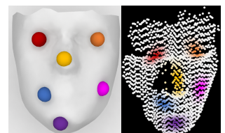
Figure 10: Point clouds.
