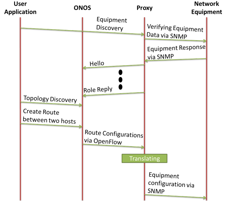
Fig. 5. Proof of Concept Global Process
