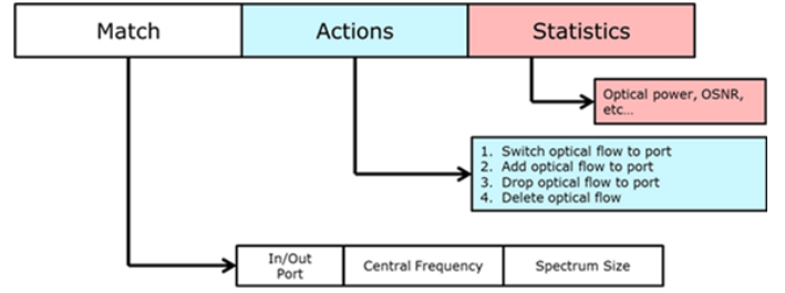
Fig. 1. Flows for wavelength switching in optical networks
