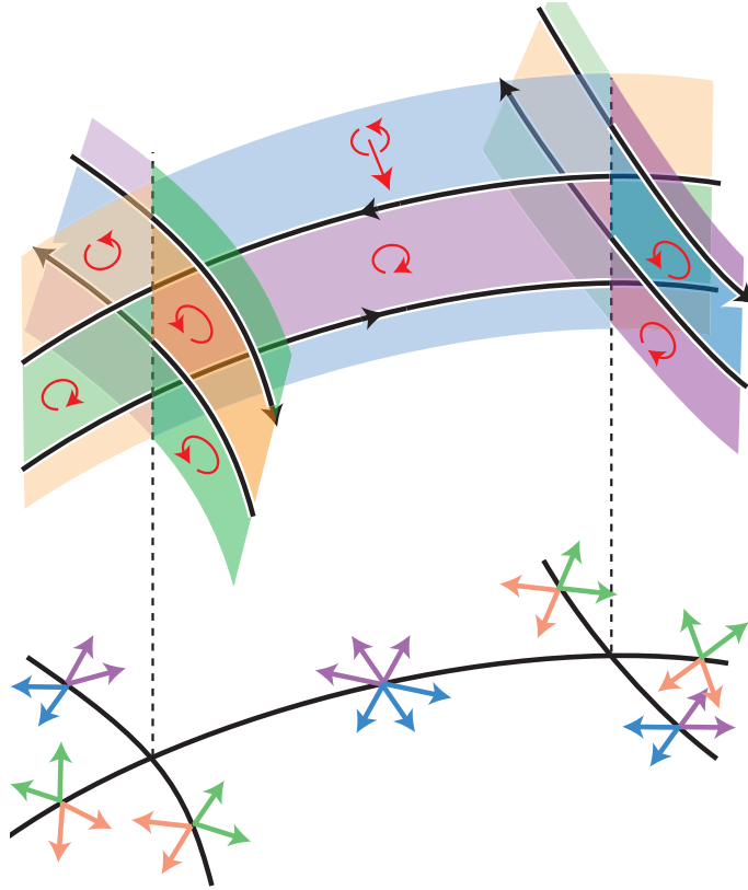
FIGURE 7. The 2-chain S_{\pm}^{\times} is half of the sum of all rectangles R^{e,\eta_e} . It is cooriented by the geodesic flow, hence oriented (in red). Its boundary, taking orientations into account, is then -\vec{\gamma} .
