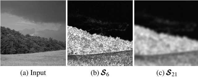
Figure 4: Descriptors scales. Small scales lead to noisy descriptors (b). Large scales lead to more homogeneous descriptors and smooth sharp texture transitions. For visualization clarity, only the first element of \mathcal{S}_r is shown (i.e. the first value of \mathbf{L}_r^1 ) but the rest of the set presents the same behavior.
