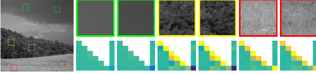
Figure 3: Texture descriptors. Patches taken from several regions of the image in Figure 2 (top) and their respective descriptors computed for the central pixel of the window (bottom). Yellow and blue values correspond to positive and negative values respectively. Patches from similar regions have similar descriptors.
