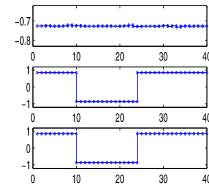
Fig. 5. Gradients of the global models. Variation of b_1
