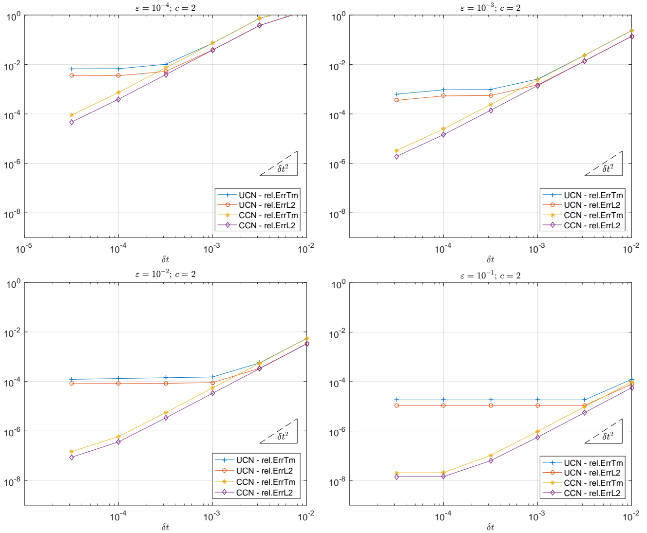
Figure 3: Evolution of the errors with respect to \delta t for c = 2 and various \epsilon
