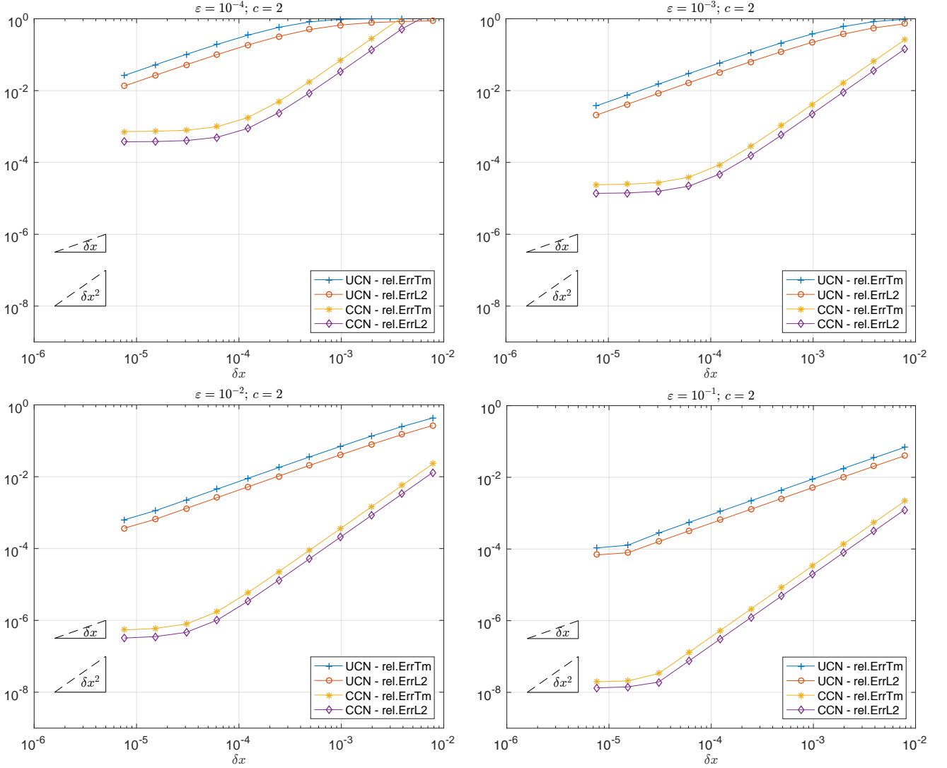
Figure 4: Evolution of the errors with respect to \delta x for c = 2 and various \epsilon
