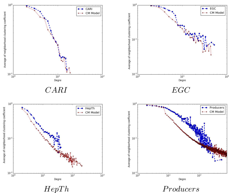
Figure 8. Corelation Degree / Clustering Coefficient of real world networks and generated networks
