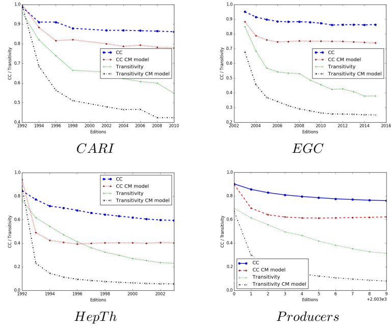
Figure 7. Clustering Coefficient and Transitivity of real world networks and generated networks
