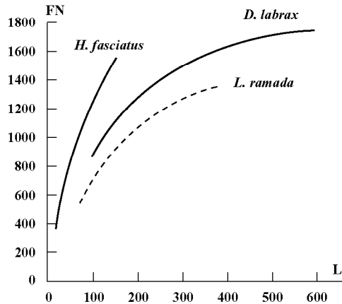
FIG. 3.— Growth curves, for three teleost species, of the total filament number (FN)(four unilateral arches) as a function of their length (in mm)(standard length (SL) for Hemichromis fasciatus ; fork length (FL) for Liza ramada (adapted from CALTRAN & SILAN, 1996) and Dicentrarchus labrax (adapted from SILAN et al. , 1987).
