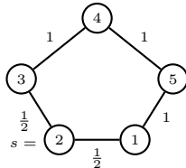
Figure 19: w_1 = w_2 = \frac{1}{2} < 1 = w_3 = \dots = w_m .
