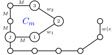
Figure 24: |E_1| \geq 2 , \sigma(N) = w_1 = w_2 = w(e) < M .
