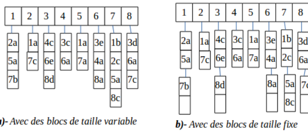
Figure 2 – Adjacency list representations of G1
