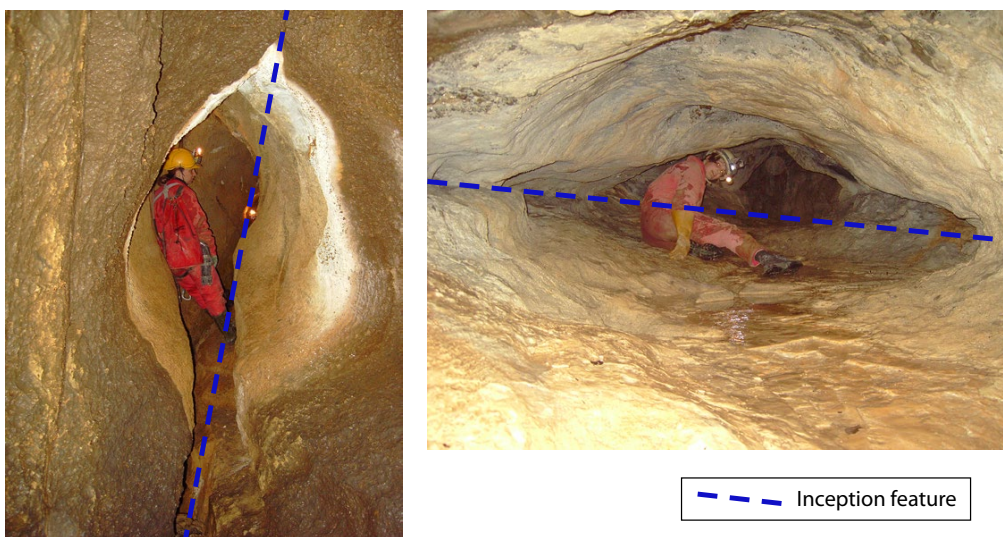
Figure 2 Examples of karst conduits showing shapes strongly elongated along inception features (left: Cave O80, Switzerland; right: Grottes aux fées, Switzerland).
