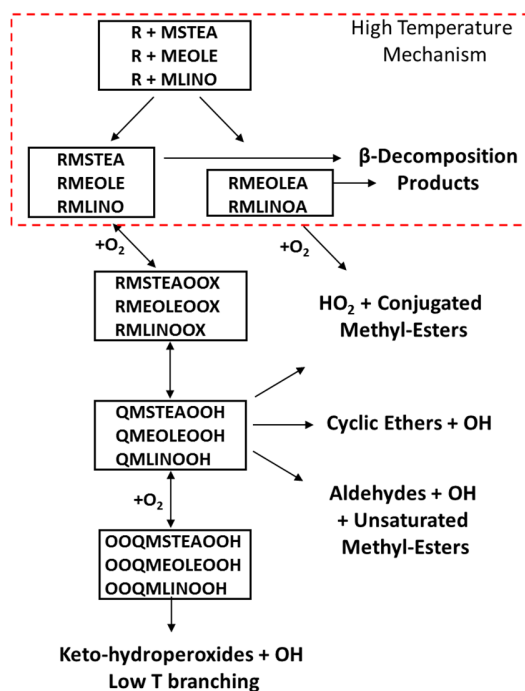
Figure 6: Lumped scheme for the three methyl-esters. Only methyl-oleate and methyl-linoleate can form the non-propagating allyl-type radicals: RMEOLEA and RMLINOA.
