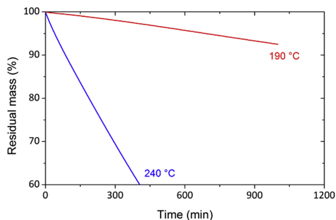
Fig. 5. TGA curves of pure Irganox 245 under N 2 atmosphere.
