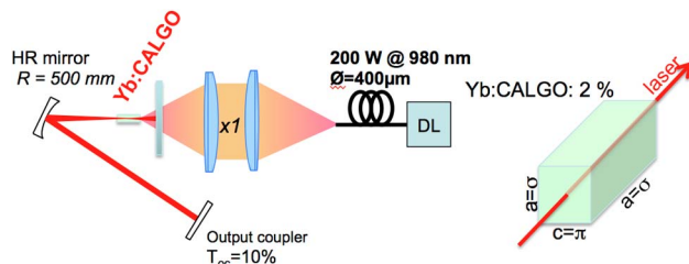
Fig. 1. Laser cavity (left). Crystal geometry (right).
