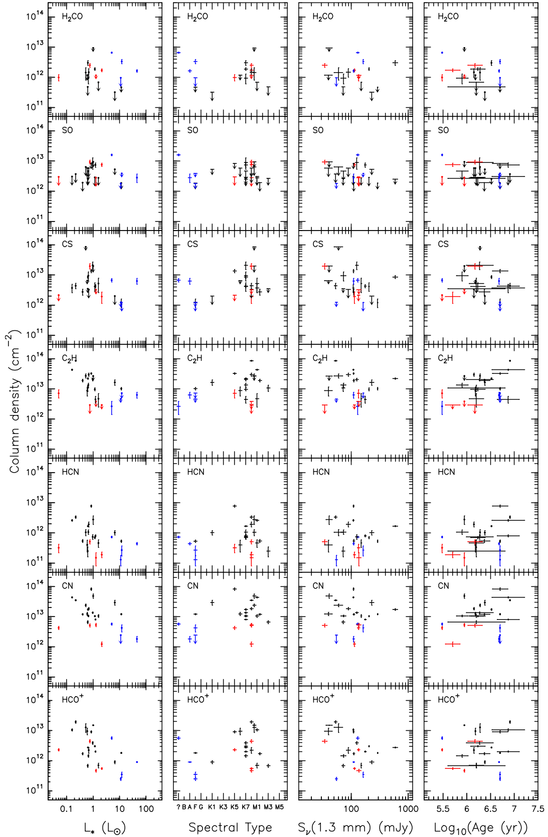
Fig. 5. Correlation plot of the column density of molecules at 300 au with stellar luminosity, spectral type, 1.3 mm flux density and stellar age. Embedded objects appear in red, H Ae stars in blue, and T Tauri stars in black. Error bars are \pm 1\sigma with limits at 2\sigma indicated by arrows.
