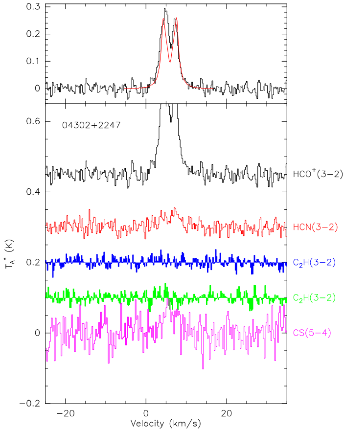
Fig. B.1. Spectra of the observed transitions toward 04302+2247.
