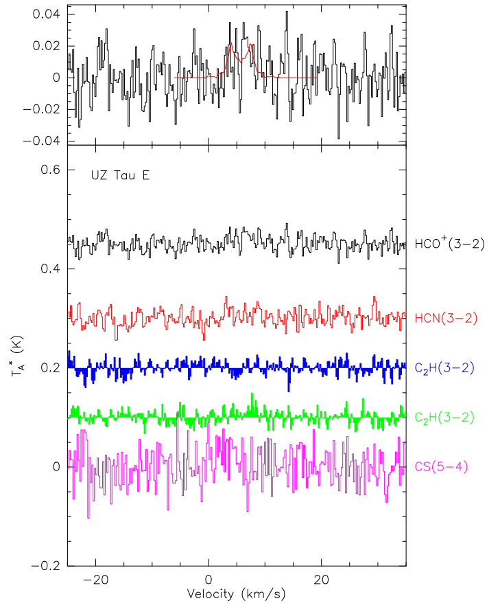
Fig. B.30. Spectra of the observed transitions toward UZ Tau E.
