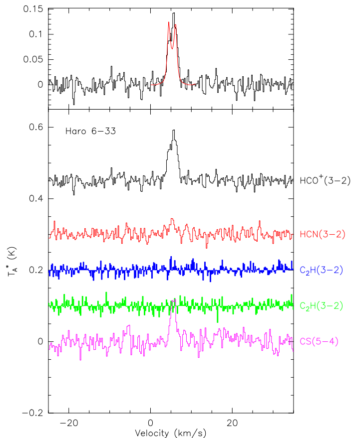
Fig. B.17. Spectra of the observed transitions toward Haro 6-33.
