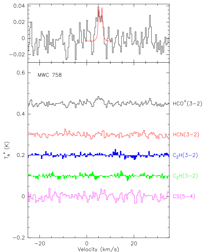
Fig. B.26. Spectra of the observed transitions toward MWC 758.
