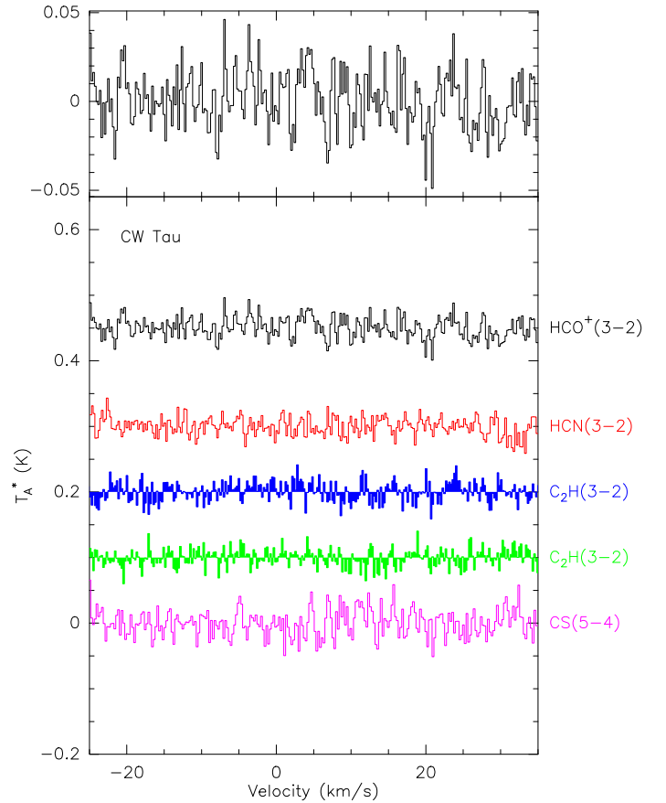
Fig. B.6. Spectra of the observed transitions toward CW Tau.
