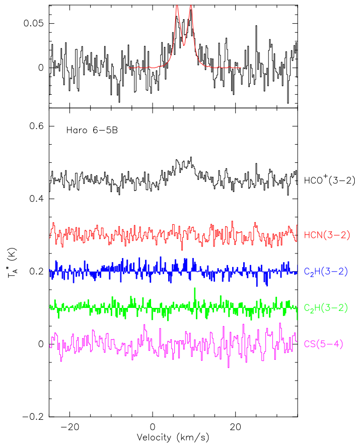
Fig. B.18. Spectra of the observed transitions toward Haro 6-5B.
