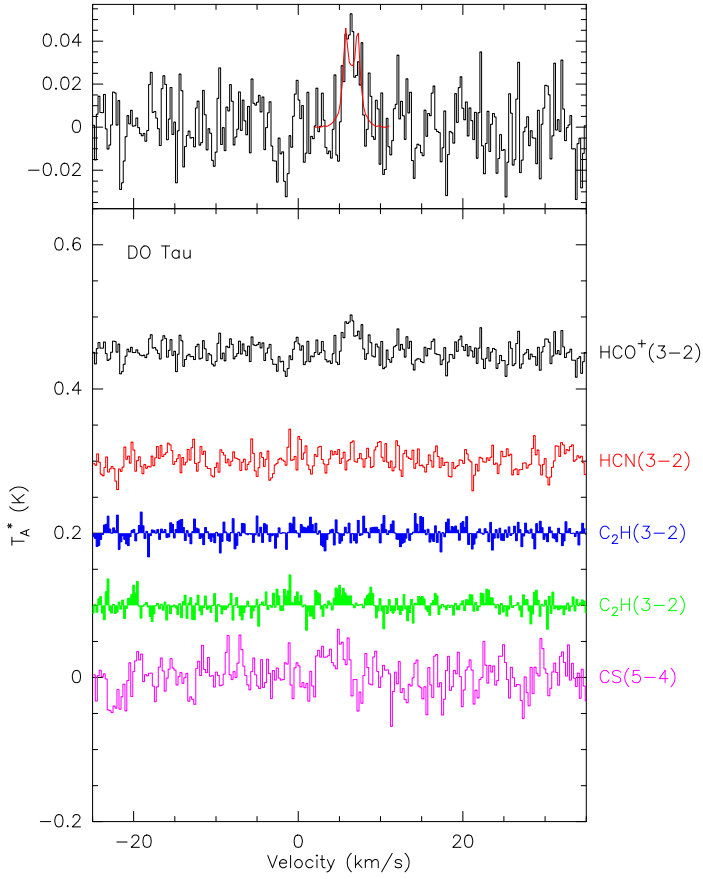
Fig. B.11. Spectra of the observed transitions toward DO Tau.
