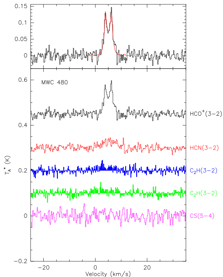
Fig. B.25. Spectra of the observed transitions toward MWC 480.
