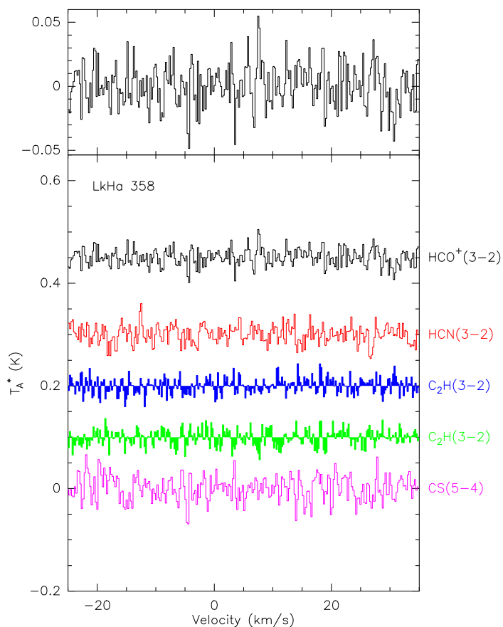
Fig. B.23. Spectra of the observed transitions toward LkH \alpha 358.
