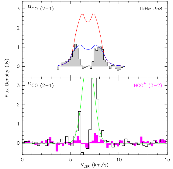
Fig. 6. Spectra of ^{12}\text{CO} , ^{13}\text{CO} , and \text{HCO}^+ toward LkH \alpha 358. Top: ^{12}\text{CO} from the interferometric measurement of Schaefer et al. (2009). The blue curve is the fitted profile based on the disk analysis made in the uv plane. The red curve uses the same disk parameters, except for the outer radius which is 250 \text{ au} instead of 170 \text{ au} . Bottom: ^{13}\text{CO}(2-1) spectrum (histogram) and \text{HCO}^+(3-2) (filled histogram). The green curve is the tentative fit of a disk component from Guilloteau et al. (2013).
