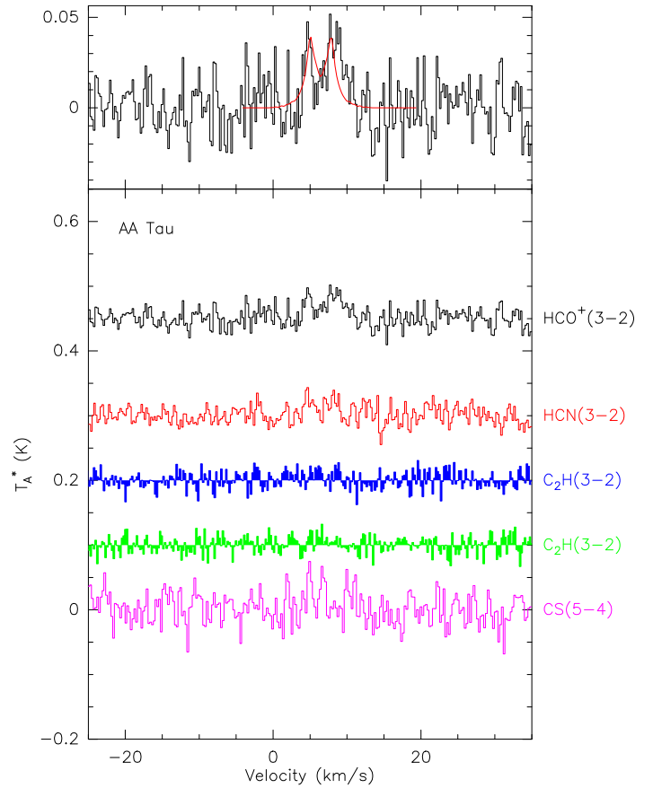
Fig. B.2. Spectra of the observed transitions toward AA Tau.
