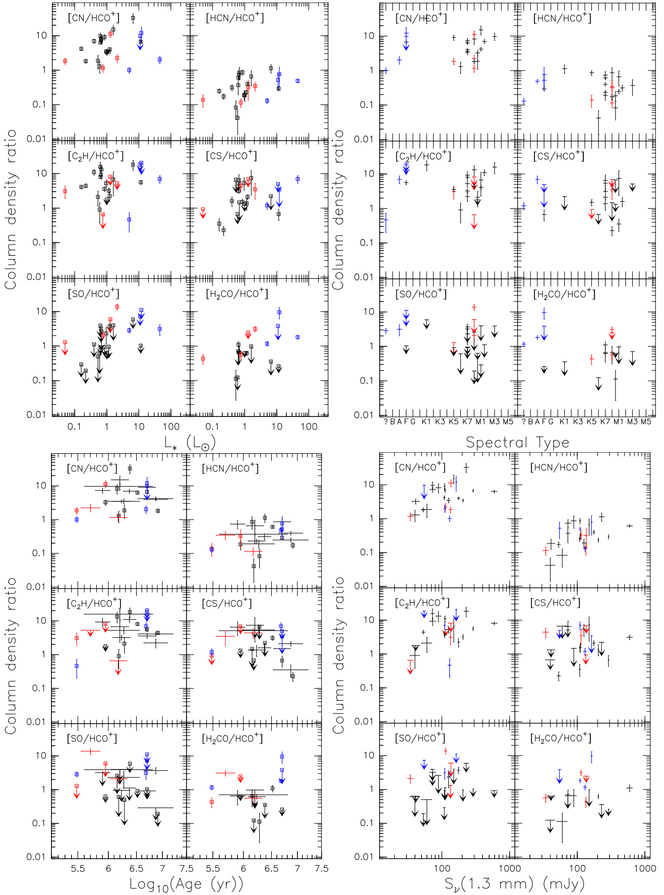
Fig. A.2. Correlation plot of the column density ratios of molecules at 300 au with stellar luminosity and spectral type, age, and 1.3 mm flux density. \text{HCO}^+ used as reference.
