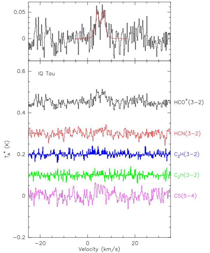
Fig. B.22. Spectra of the observed transitions toward IQ Tau.
