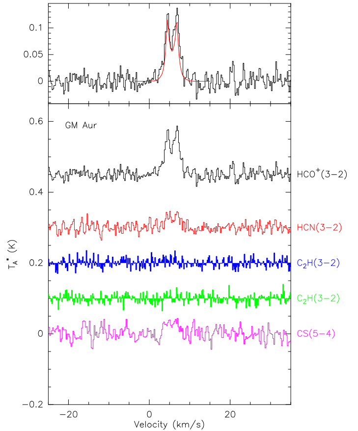
Fig. B.14. Spectra of the observed transitions toward GM Aur.
