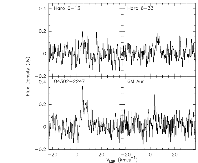
Fig. 4. Averages of the SO( 6_5-5_4 ) and SO( 6_7-5_6 ) spectra resampled to a common velocity scale.
