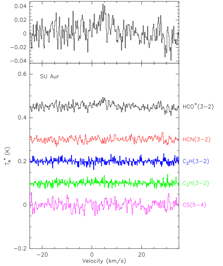
Fig. B.29. Spectra of the observed transitions toward SU Aur.
