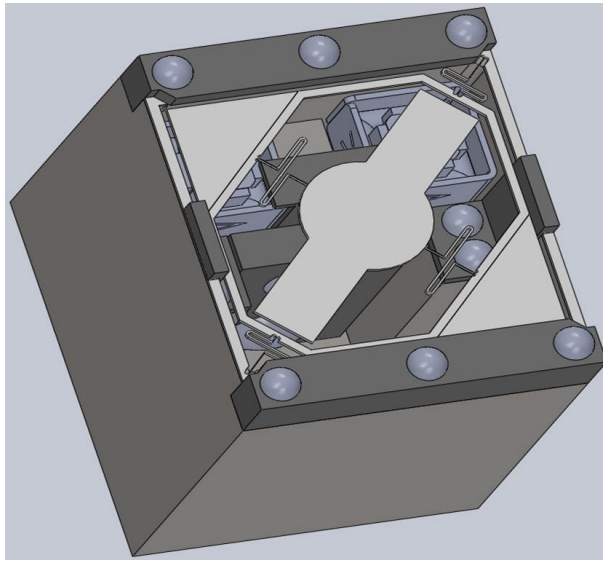
Figure 3: The concept of Squipabot for beam steering with dimension about 8 mm x 10 mm x 12 mm.
