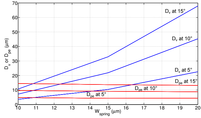
Figure 8: The effect of the spring width on D_{pe} and D_v .
