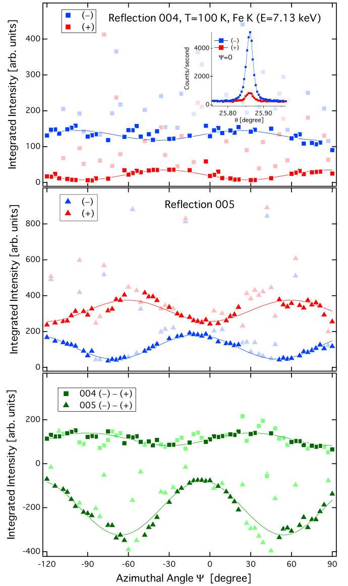
FIG. 6. The integrated intensity of forbidden reflections 004 (top panel) and 005 (middle panel) observed at the Fe K absorption edge ( E = 7.13 keV) and temperature T = 100 K as a function of \Psi . The inset of the top panel shows rocking curves observed at \Psi = 0 for (+) and (-) helicity of the incident beam. Red squares (triangles) show the integrated intensity measured by the incident beam with the (+) helicity for reflection 004 (005) and blue squares (triangles) show that measured by the incident beam with the (-) helicity for reflection 004 (005). The bottom panel shows the difference intensity (-) - (+) between the two helicity states. The cosine curves are results of fit to the data with Eq. (14) for the top and middle panels, and fit to the data with Eq. (18) for the bottom panel. The points colored faintly are strongly influenced by the multiple scattering effect, and are removed for the fitting.
