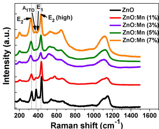
Fig. 2. Room temperature Raman spectra of ZnO and Mn-doped ZnO nanoparticles.
