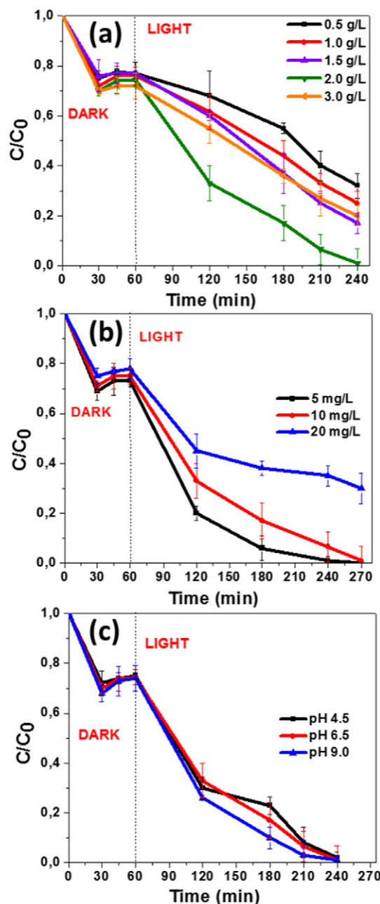
Fig. 7. Influence of (a) the amount of catalyst, (b) the dye concentration and (c) the pH of the Orange II solution on the photocatalytic activity of ZnO:Mn (3%) particles.
