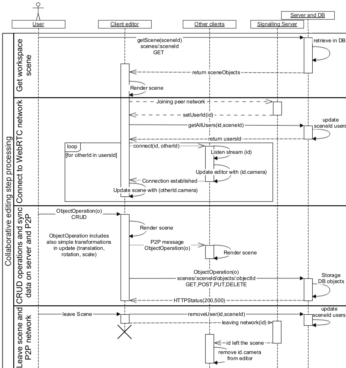
Figure 5: Sequence diagram of collaborative communication process
