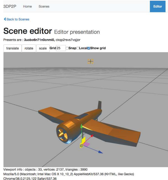
Figure 6: Editor interface
