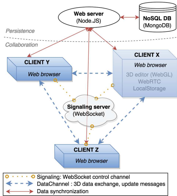
Figure 4: System overview
