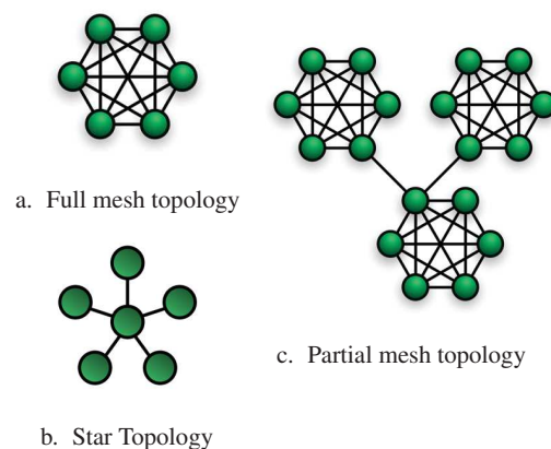
Figure 1: Peer-to-peer topologies
