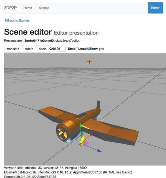
Figure 1: Editor presentation
