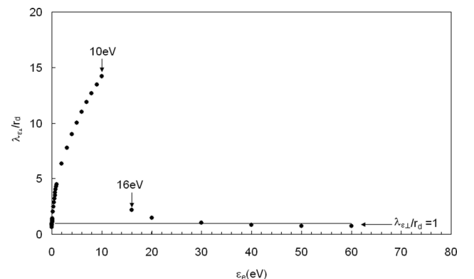
FIG. 3. Ratio of the electron energy relaxation length on the disturbed probe length versus electron energy in \text{H}_2 magnetoplasma. The straight line indicates the ratio equal to 1.
