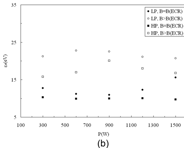
FIG. 6. Electron density (a) and mean energy (b) versus incident power, in resonance ( B = B(\text{ECR}) ) and off resonance ( B > B(\text{ECR}) ) conditions, at the two pressures LP (0.38 Pa) and HP (0.62 Pa) and at t = 300 \mu s .
