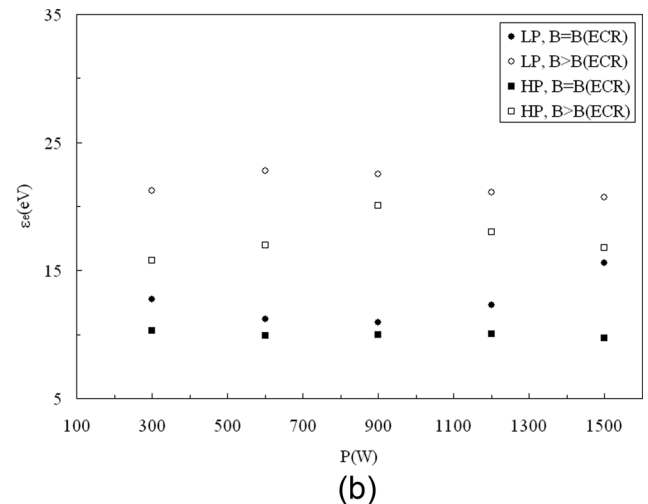
FIG. 6. Electron density (a) and mean energy (b) versus incident power, in resonance ( B = B(\text{ECR}) ) and off resonance ( B > B(\text{ECR}) ) conditions, at the two pressures LP (0.38 Pa) and HP (0.62 Pa) and at t = 300 \mu\text{s} .
