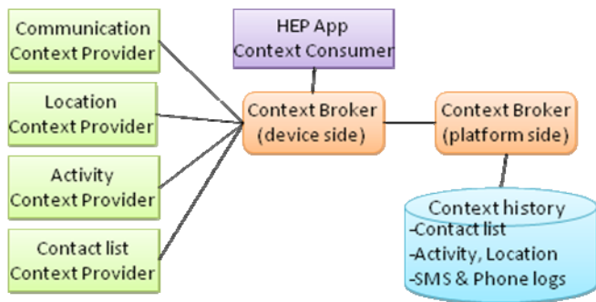
Figure 3: HEP architecture
