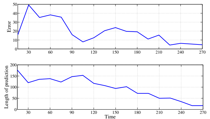
Figure 14. Error between predictions and real observations (top) and the length of the predictions (bottom).
