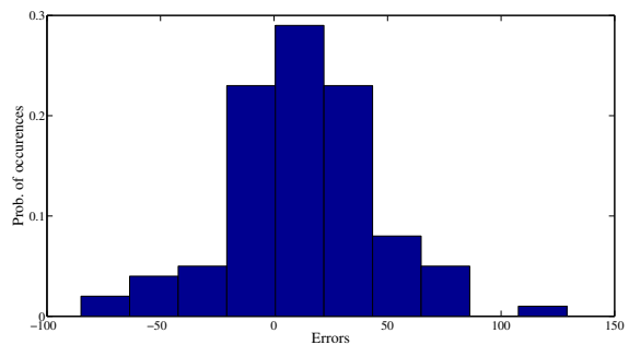
Figure 19. Distribution of errors of the RUL's estimates for the second dataset.
