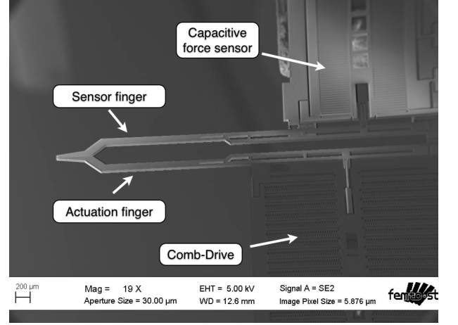
Figure 6: Micro-gripper FTG-30 (image acquired with SEM). The left finger can be actuated through a comb-drive mechanism.
