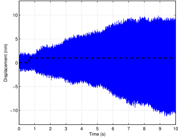
Figure 13: Displacement measurement of silicon cantilever under the influence of a external source of noise (loudspeaker). A sinusoidal wave with frequency matching the sample's first mode is applied. The black dotted line indicates when the external disturbance begins.
