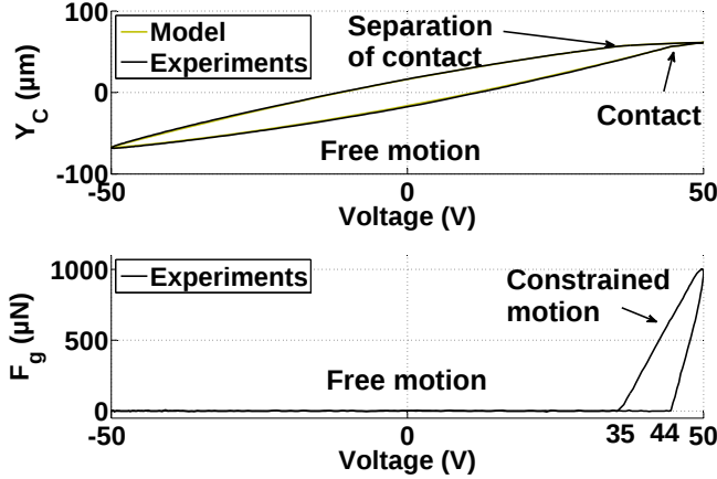
Fig. 13: Comparison between the model of the displacement of the TSFM tips C given in (11) and experimental measurements. The measurement force is also shown.
