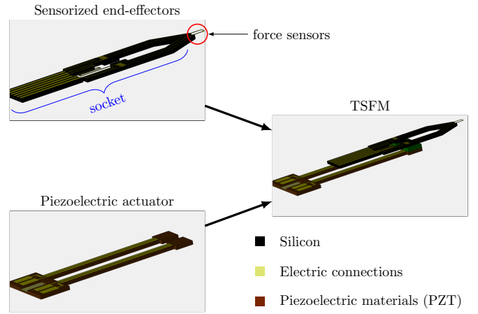
Fig. 2: Integration of the sensorized end-effectors into a piezoelectric actuator to realize the TSFM.
