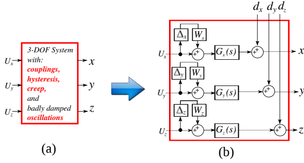
Figure 14: (a): the nonlinear, oscillating and coupled 3-DOF system. (b): approximation into 3 monovariable systems with external fictive disturbance.
