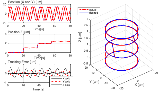
Figure 21: Helix trajectory tracking.
