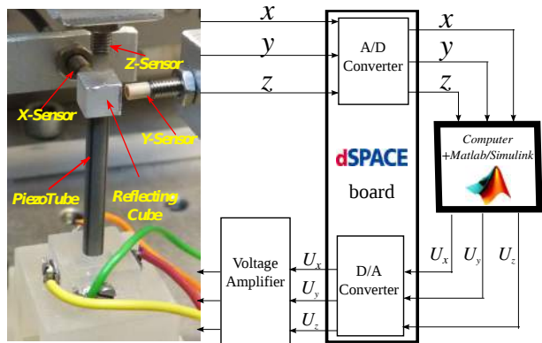
Figure 10: Experimental setup description.
