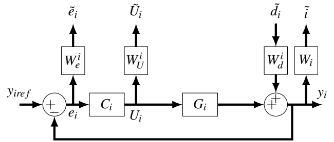
Figure 7: The representation from which the standard H_\infty problem is defined (equivalent representation of the scheme of Fig. 6 in terms of stability condition).
