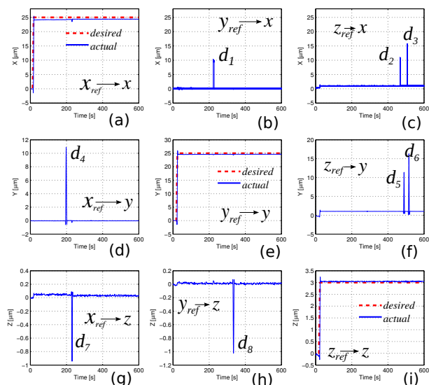
Figure 19: Verification of the creep for the closed-loop.
