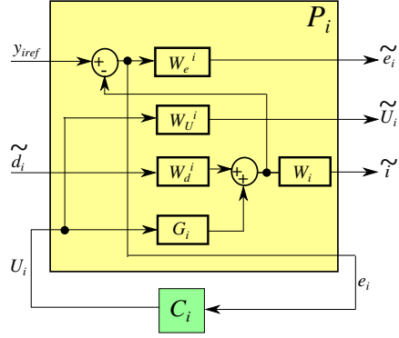
Figure 8: The standard scheme block diagram for each axis i .
