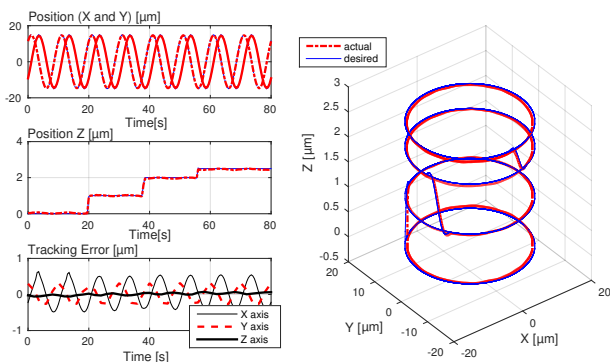
Figure 21: Helix trajectory tracking.
