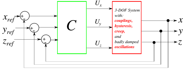
Figure 17: The closed-loop control of the 3-DOF positioner.
