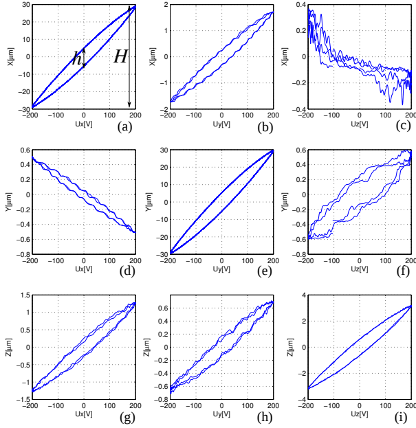
Figure 11: Hysteresis characterization with input sinusoidal signals of amplitude 200V and of frequency 0.1Hz. Notations h and H in (a) are used later for computation of numerical values of hysteresis.
