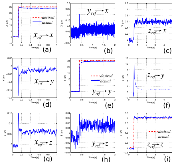
Figure 20: Verification of the transient parts for the closed-loop.
