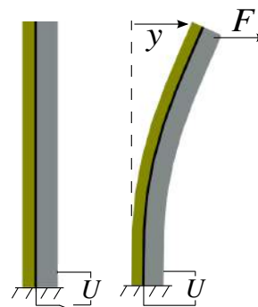
Figure 1: Deflection y of a piezoelectric cantilever driven by a force F and a voltage U .
