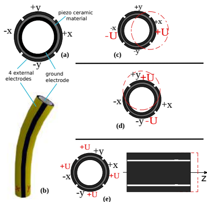
Figure 9: Piezoelectric tube structure and operation: (a) Top view, showing four external electrodes and an internal ground electrode, separated by piezoelectric material; (b) A perspective view of the piezoelectric tube; (c) deflection along X axis; (d) deflection along Y axis, and (e) elongation along Z axis.
