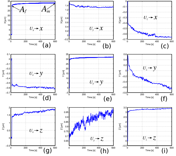
Figure 12: Creep characterization: step responses obtained with input steps of amplitude 200V and observed over a period of 600s. Notations A_f and A_m in (a) are used later for computation of numerical values of creep.
