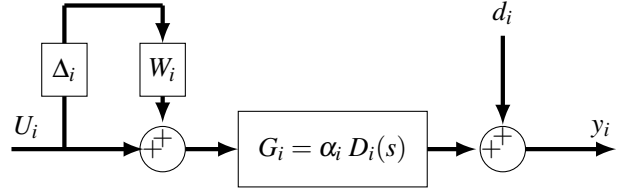
Figure 5: Implementation of the proposed model for axis i ( 1 \leq i \leq n ): cross-couplings, creep and direct hysteresis offsets are included in the disturbance d_i . \Delta_i represents the normalized model uncertainty ( \|\Delta_i\|_\infty \leq 1 ).
