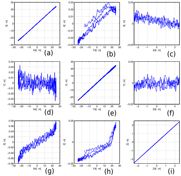
Figure 18: Verification of the hysteresis for the closed-loop.
