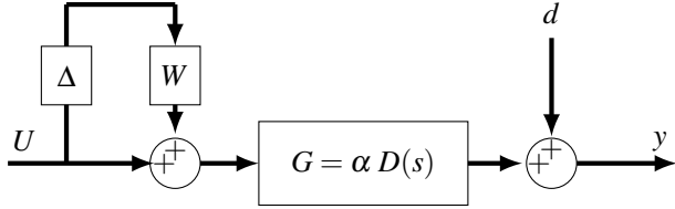
Figure 3: Implementation of the linear and dynamic model for the deflection y of a piezoelectric actuator driven by a voltage U . \Delta represents the normalized model uncertainty ( \|\Delta\|_\infty \leq 1 ) and d the disturbance to the system, which includes the creep and hysteresis offset.
