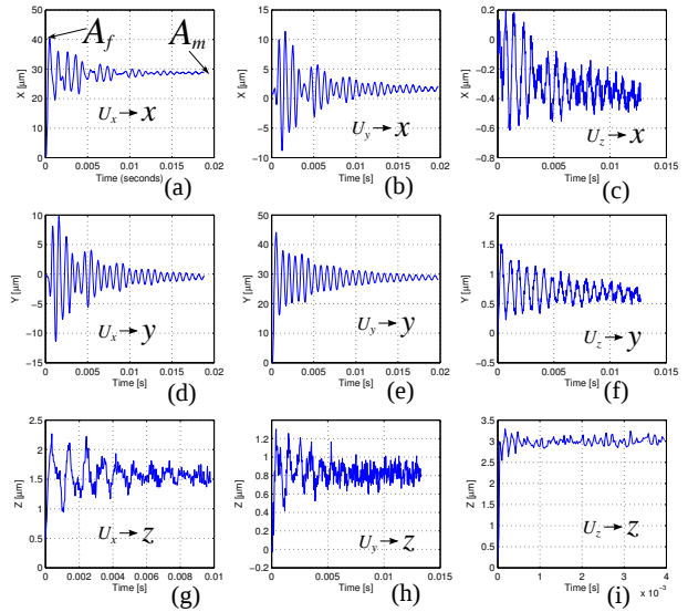
Figure 13: Dynamics characterization: transient responses obtained with step inputs of amplitude 200V and observed during 20ms. Notations A_f and A_m in (a) are used later to numerically quantify the oscillations.
