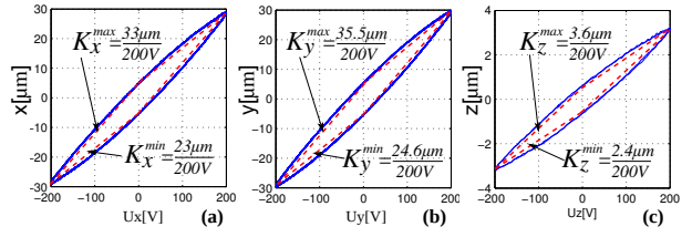
Figure 15: Experimental hysteresis curves (blue-solid line), quadrilateral modeling (red-dashed line) and numerical values of slopes K^{max} and K^{min} , for each axis: (a), (b) and (c) represent hysteresis x vs U_x , y vs U_y and z vs U_z , respectively.
