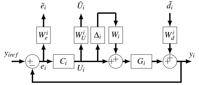
Figure 6: The closed-loop system augmented by the proposed weightings. \Delta_i represents the normalized model uncertainty ( \|\Delta_i\|_\infty \leq 1 ).
