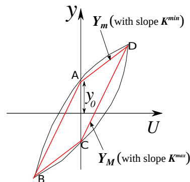
Figure 2: Quadrilateral modeling of hysteresis.
