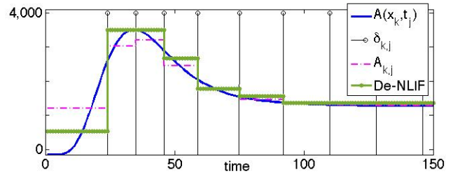
FIGURE 5 – NLIF-based de-quantization.
