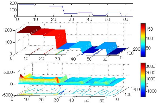
FIGURE 2 – Top : 1D spatial signal f(x) . Middle : 1D spatial filter f(x)\mathbb{1}_{[0, \Delta T]}(t) flashed for a given time \Delta T . Bottom : Spatiotemporally filtered signal A(x_k, t_j) .
