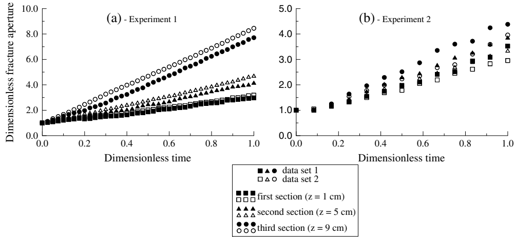
Figure 3. Evolution of the dimensionless fracture aperture versus time along three sections perpendicular to the mean flow for: (a) Q_v = 1.0 mL/h and (b) Q_v = 15 mL/h.
