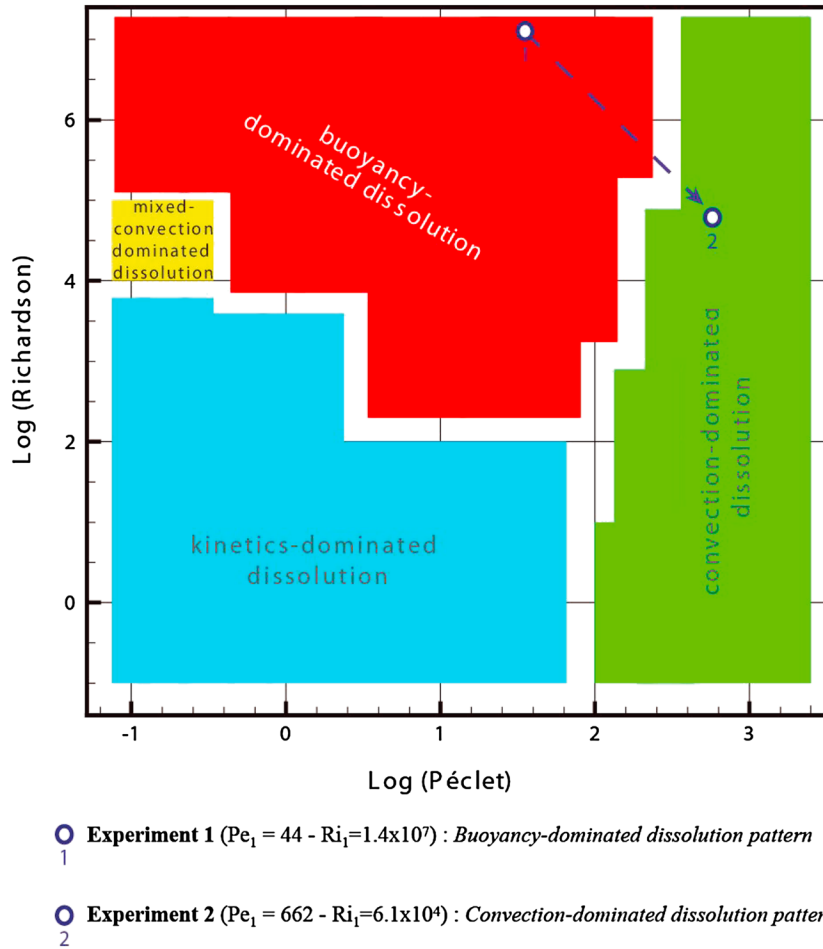
Figure 9. Plot illustrating the empirically-classified dissolution regimes for the estimated value of the experimental Damköhler number ( Da=4 ). The points 1 and 2 correspond to the experiments conducted in this paper.
