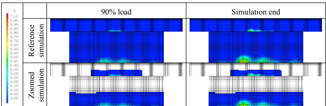
Figure 3 : Damage profiles at 90% load and at the end of the simulation.
