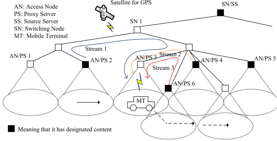
Figure 1: Proxy server handoff architecture for mobile IPTV services.
