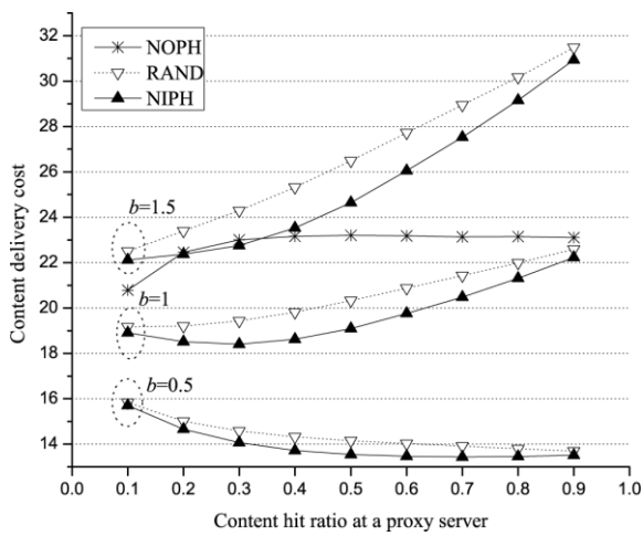
Figure 3: Content delivery cost (R(t_1+t_2+\dots+t_i) = 4; C_{ph} = 1)
