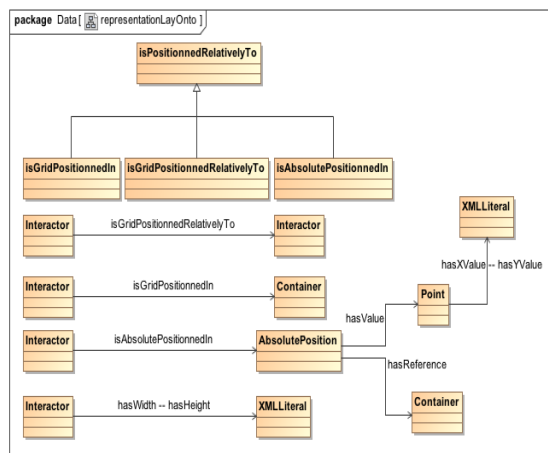
Figure 2. LayOnto
