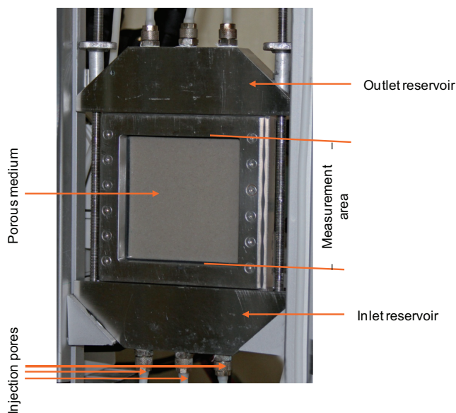
Figure 2. Flow cell features.
