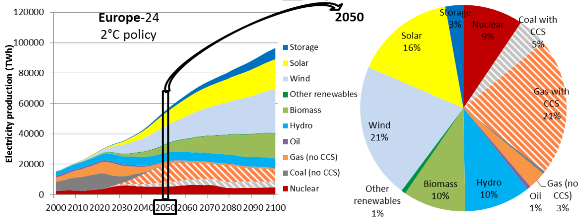
Figure C-1: European power supply in the 2°C policy scenario (POLES+EUCAD).
