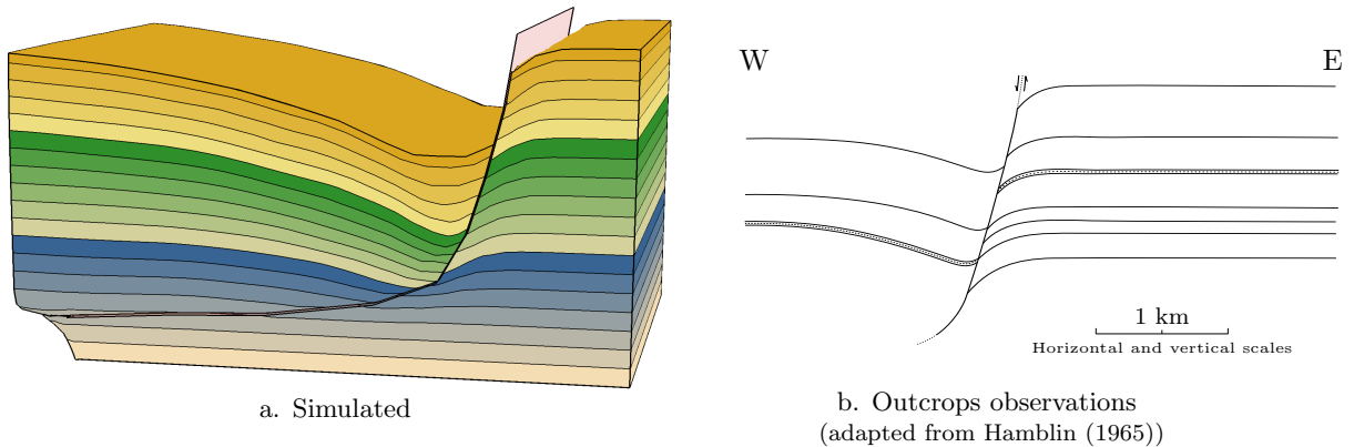
Figure 10: Listic fault displacement field. This figure presents the results of the deformation associated with a listric fault. The numerical model (a) is designed to reproduce typical folds observed in the flanks of natural listric faults (b): a normal drag, present in both blocks, and a reverse drag, in the hanging wall only, forming a roll-over anticline. The normal drag is interpreted here as the heritage of a fault-propagation fold (Reches and Eidelman, 1995). It is obtained by adapting the attenuation profile to produce a continuous shear parallel to the fault applied at the beginning of the deformation process. The hanging wall is progressively affected by a displacement vector field following eq. (2), until a global displacement of 250m to the West is reached (see algorithm Fig. 9). This process produces a roll-over anticline. It is not imposed explicitly but represents an emergent character implied by the fault geometry. The simulated roll-over anticline and the normal drag (a) are similar to those observed in the natural fault depicted in Hamblin (1965) (b). Note that the fault in this example has been chosen for its well identified normal drag and roll-over anticline. This case may not be representative of most listric faults due to the accentuated difference of dip between the top and bottom parts of the fault.
