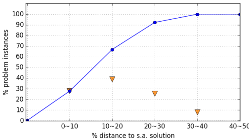
Fig. 5. Distance between solution costs from simulated annealing solutions and greedy heuristics group on problem instances where simulated annealing solutions were better.
