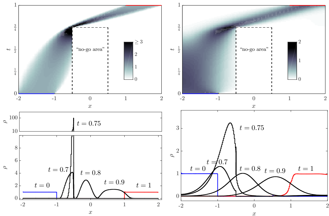
FIG. 4. The example from Section 5.2. Density \rho in space-time (top) and its temporal snapshots (bottom) with diffusion coefficient \nu = 10^{-1} (left) and \nu = 1 (right).
