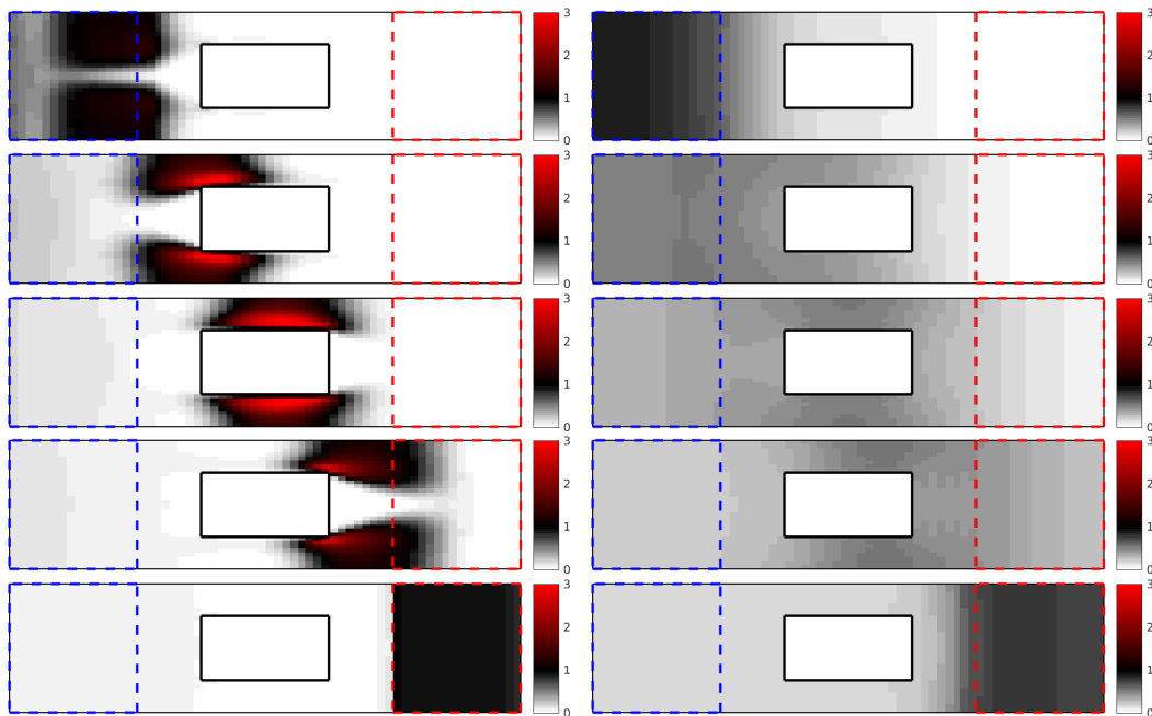
FIG. 5. The example from Section 5.3. Temporal snapshots \rho_h(t, \cdot) of the computed density at t = n/13 for n = 1, 4, 7, 10, 13 (top to bottom). Diffusion coefficient \nu = 10^{-1} (left) and \nu = 1 (right).
