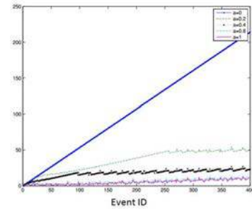
Figure 8. Standard Deviation Different \alpha
