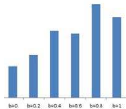
Figure 11. Average Waiting Time Different \beta
