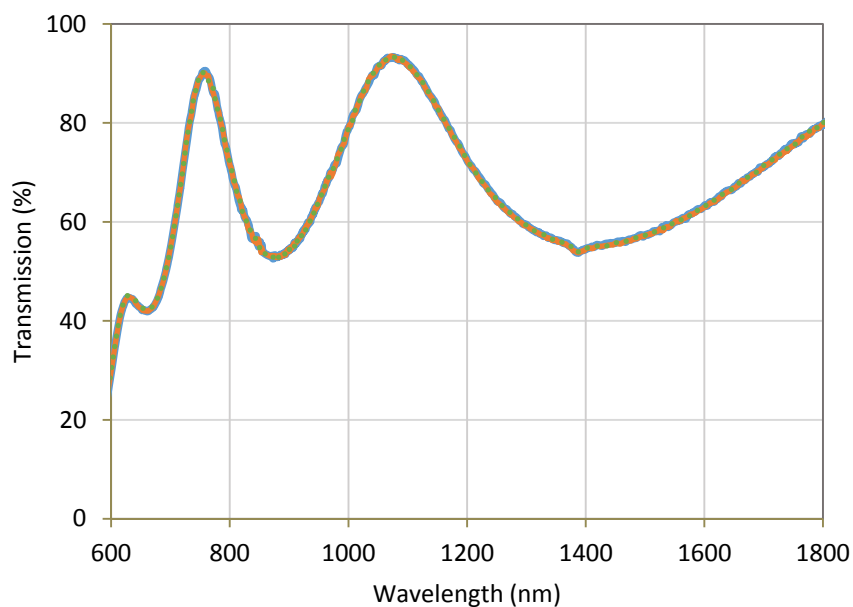
Figure 10: Spectral dependence of the transmission measured on an unexposed sample at different duration of storage in dark: in blue – 0 days, in orange – 10 days, in green – 20 days and black points - 70 days.
