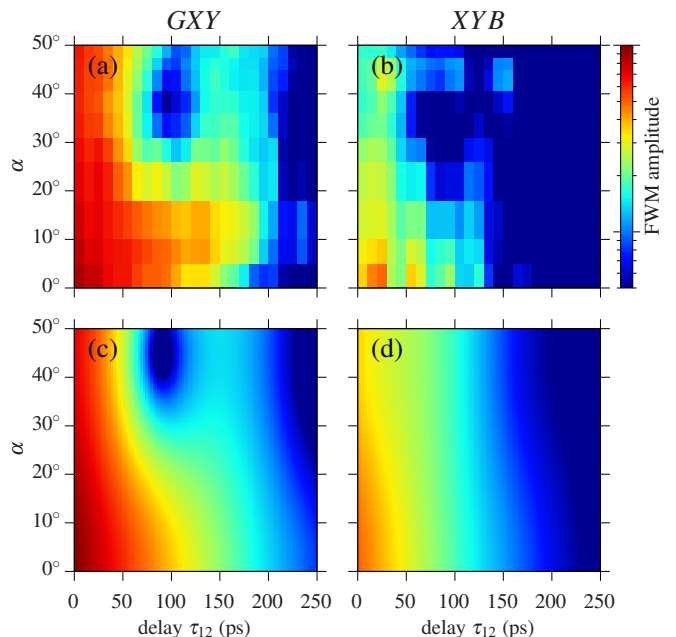
FIG. 3. Coherence dynamics for co-linear excitation. (a,b) Measurements and (c,d) calculations of the coherence dynamics as function of delay \tau_{12} and polarization angle \alpha for co-linear excitation for (a,c) the GXY transition and (b,d) the XYB transition.
