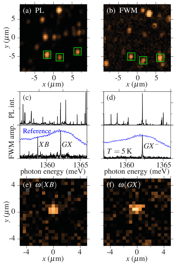
FIG. 10. Sample characterization. Hyperspectral image of the sample for (a) PL and (b) FWM measurements. (c,d) PL and FWM spectra of a single QD. Blue indicates the spectrum of the laser pulse as reference. (e,f) Hyperspectral FWM image of of XB and GX transition.
