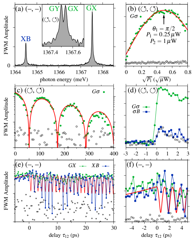
FIG. 2. Quantum beats. (a) Two-pulse FWM spectra of a single QD for co-linear polarization. Inset: Zoom in on the exciton line for co-circular polarization. (b) FWM signal as function of excitation intensity \sqrt{P_1} . (c) FWM signal as function of time delay \tau_{12} for co-circularly polarized excitation. (d) Zoom-in of (c) around \tau_{12} = 0 . (e) and (f) FWM signal as function of \tau_{12} for linear polarization with \alpha = 0^\circ . Green dots and blue squares: experimental data; gray circles: indication of noise level; red lines: theoretical calculation.
