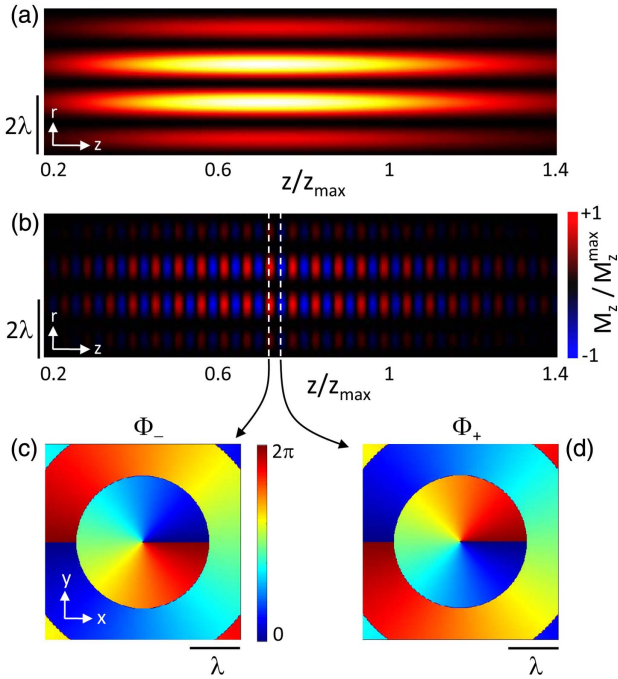
Fig. 7. (a) Total intensity near the z axis of a hollow beam with self imaged orbital angular momentum generated from an incident \mathbf{e}_+ Laguerre Gaussian beam of order l = 1 . (b) Orbital angular momentum density M_z(r, z) color map, where luminance is proportional to the total intensity shown in panel (a). Transverse phase profiles of the \mathbf{e}_- and \mathbf{e}_+ polarized components are shown in (c) and (d), respectively.
