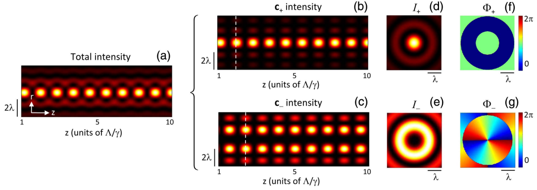
Fig. 3. (a) Total intensity distribution near the z axis in the case of a \mathbf{c}_+ polarized incident plane wave. The intensity distribution of the \mathbf{c}_\pm polarized components are shown in (b) and (c), whereas the transverse intensity ( I_\pm ) and phase ( \Phi_\pm ) profiles associated with a local intensity maximum (see dashed vertical lines) are shown in (d), (e) and (f), (g).
