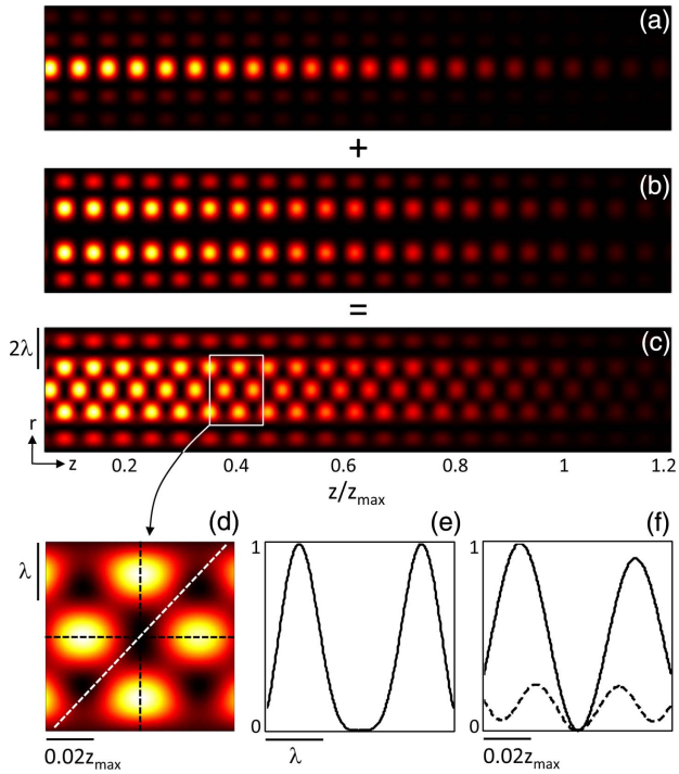
Fig. 5. Same as in Fig. 4 in the case of two contracircularly polarized fundamental Gaussian beams ( l = 0 ) for a ratio of amplitude \simeq 2.1 between the \mathbf{c}_\sigma and \mathbf{c}_\sigma polarized incident beams.
