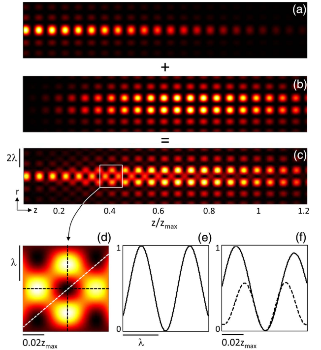
Fig. 4. Intensity distribution near the z axis of the \mathbf{c}_\sigma polarized component of the field in the case of incoherent superposition of two Laguerre Gaussian beams: (i) a \mathbf{c}_\sigma ( \sigma = \pm 1 ) polarized beam of order l = 0 and (ii) a \mathbf{c}_{-\sigma} polarized beam of order l = \sigma . (a) Beam (i) alone. (b) Beam (ii) alone. (c) Beams (i) and (ii) together for a ratio of amplitude E_\sigma/E_0 \simeq 4.4 . (d) Enlargement of the region near z/z_{\max} \simeq 0.4 that corresponds to an optical bottle. (e) Normalized transverse intensity profile; see vertical black dashed line in (d). (f) Solid curve, normalized longitudinal intensity profile [see horizontal black dashed line in (d)]; dashed curve, intensity profile along the diagonal white dashed line in (d).
