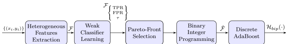
Figure 3: Proposed cascade node training scheme using heterogeneous pool of features and binary integer programming.
