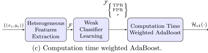
Figure 9: Block diagrams of three other nodal strong classifier learning approaches.
