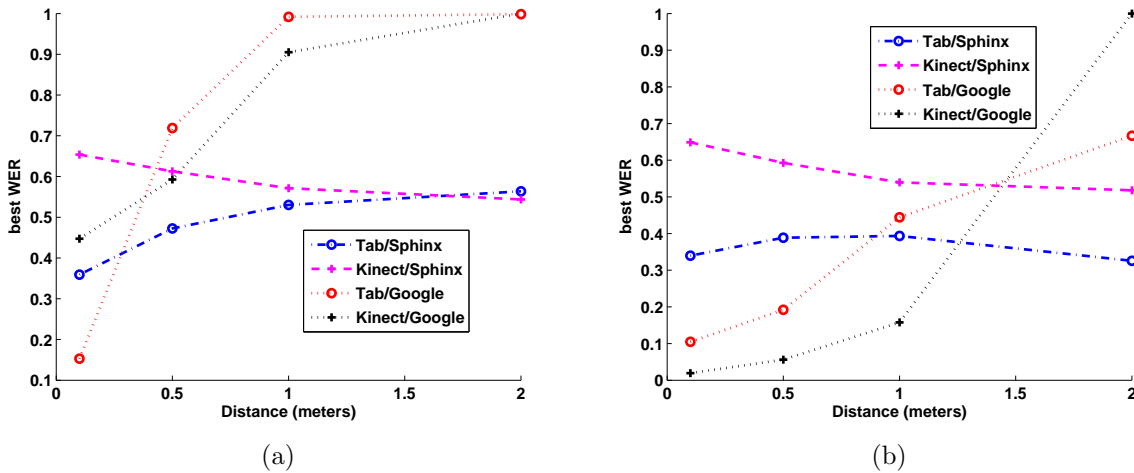
Fig. 17: (a) Performances of each combination considering T-WER. For (a) and (b) only the best WER is displayed for readability reasons. (b) Performances of each combination considering U-WER. Curve behaviors are the same for likely WER and worst WER.
